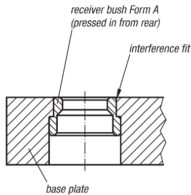
recommended installation
